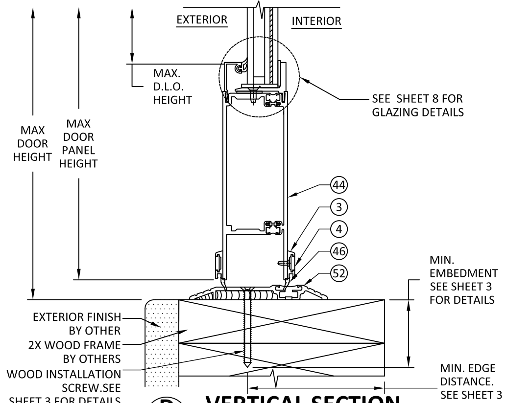
D 4 VERTICAL SECTION 500T DOOR & TRIFAB 451T SUBFRAME SILL-2X WOOD FRAME
