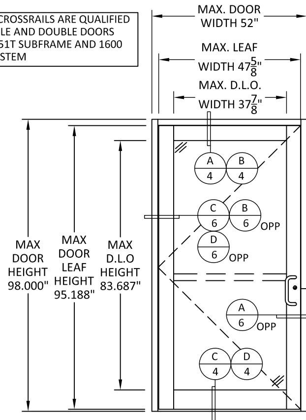
ELEVATION 500T THERMAL SINGLE DOOR WITH 451T SUBFRAME
