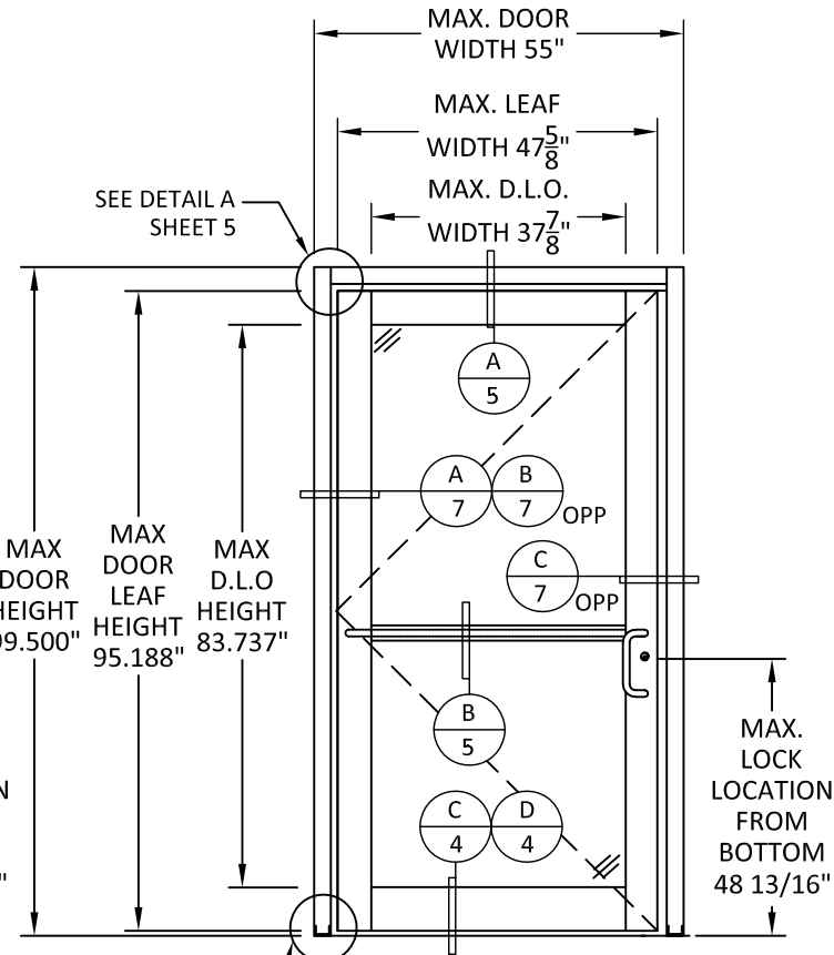
ELEVATION 500T THERMAL SINGLE DOOR WITH 1600 WALL SYSTEM
