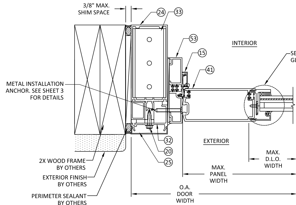
C HORIZONTAL SECTION 7 500T DOOR & 1600 WALL SYSTEM JAMB
