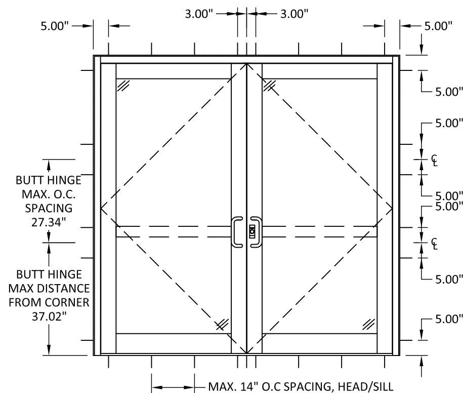
ANCHOR LAYOUT
