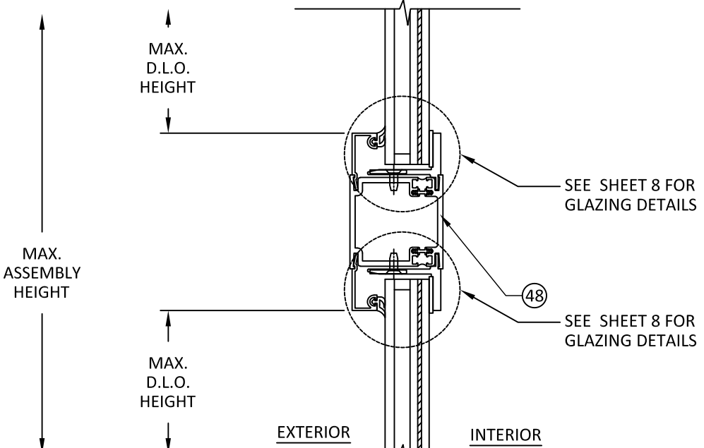
B 5 VERTICAL SECTION CROSSRAIL THERMALLY BROKEN
