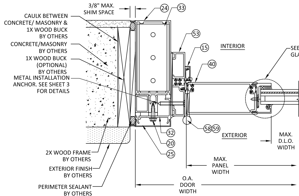
A HORIZONTAL SECTION 7 500T DOOR & 1600 WALL SYSTEM JAMB
