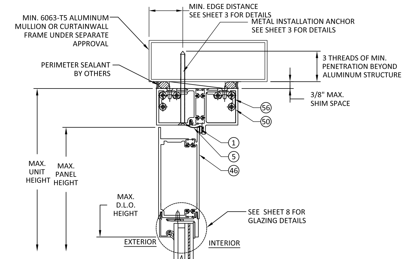
A 4 VERTICAL SECTION 500T DOOR & TRIFAB 451T SUBFRAME HEAD-METAL STRUCTURE
