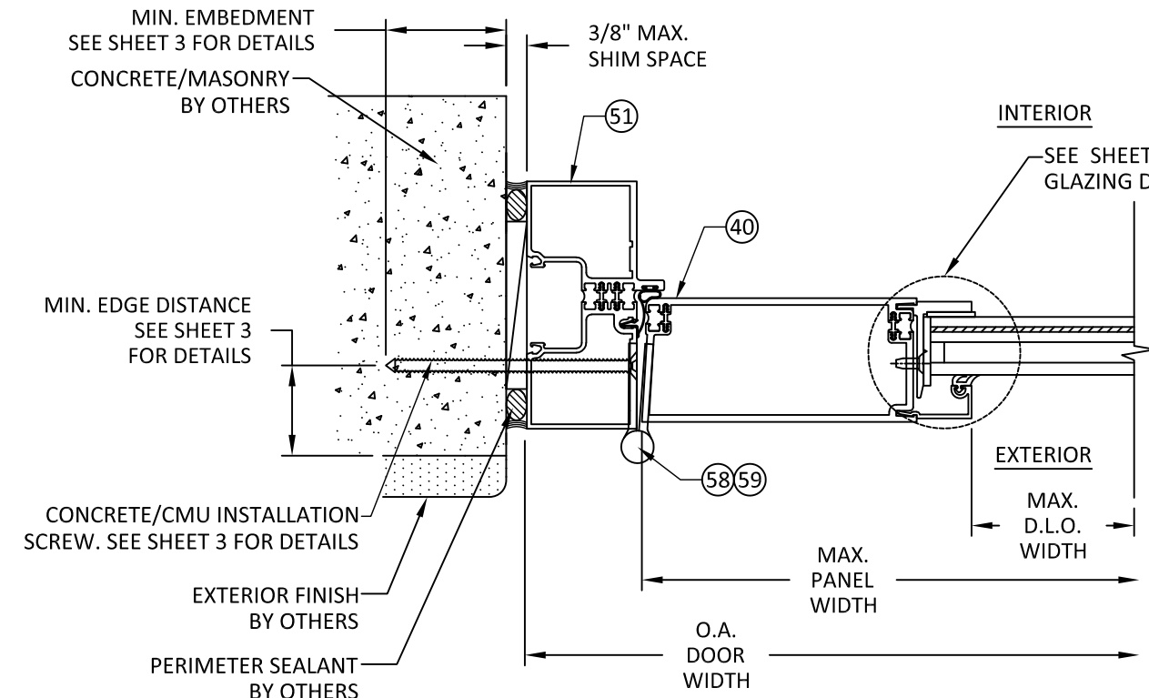
C HORIZONTAL SECTION 6 500T DOOR & TRIFAB 451T SUBFRAME JAMB-CONCRETE/MASONRY
