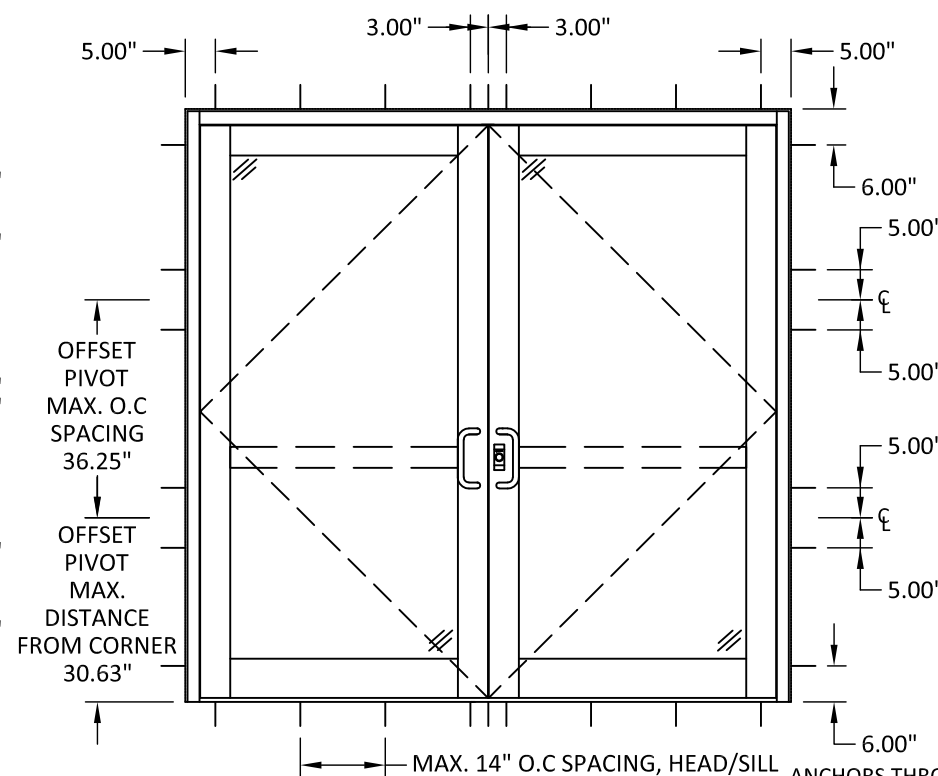
ANCHOR LAYOUT
