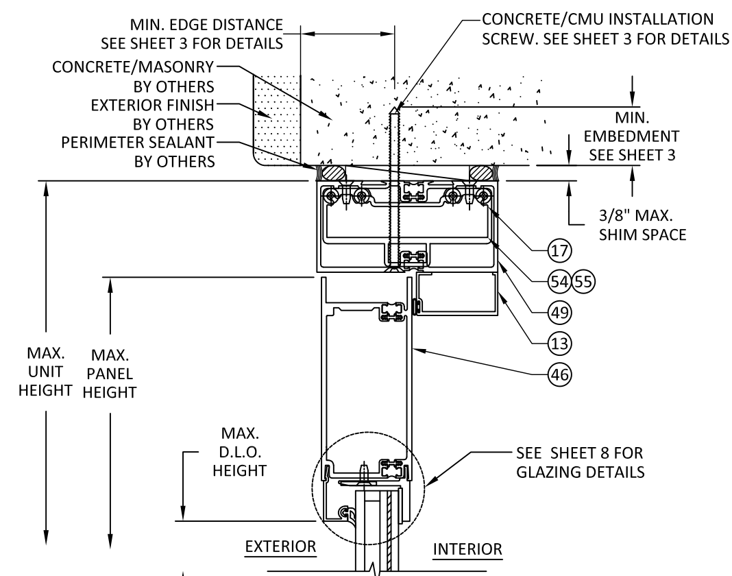
B 4 VERTICAL SECTION 500T DOOR & TRIFAB 451T SUBFRAME HEAD-CONCRETE/CMU
