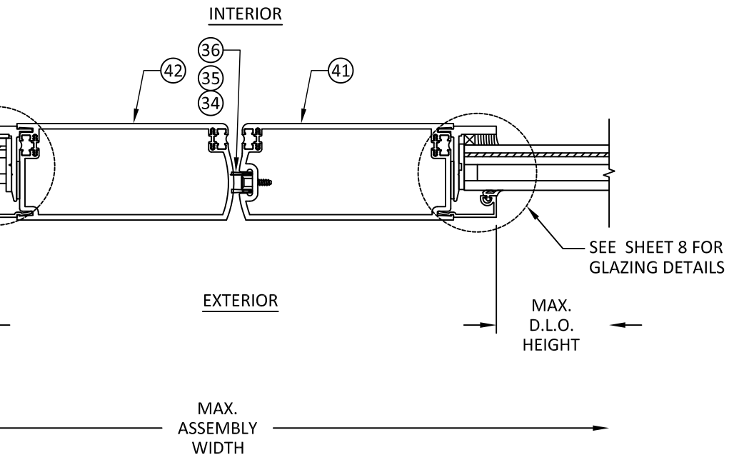
D HORIZONTAL SECTION 7 ASTRAGAL THERMALLY BROKEN
