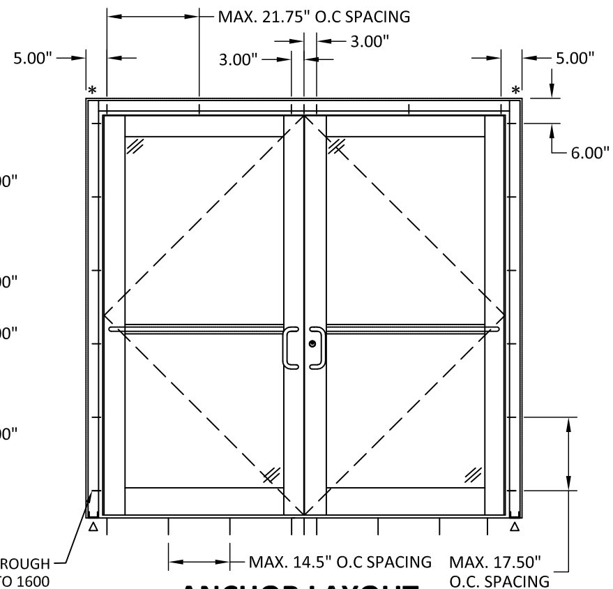
ANCHOR LAYOUT
