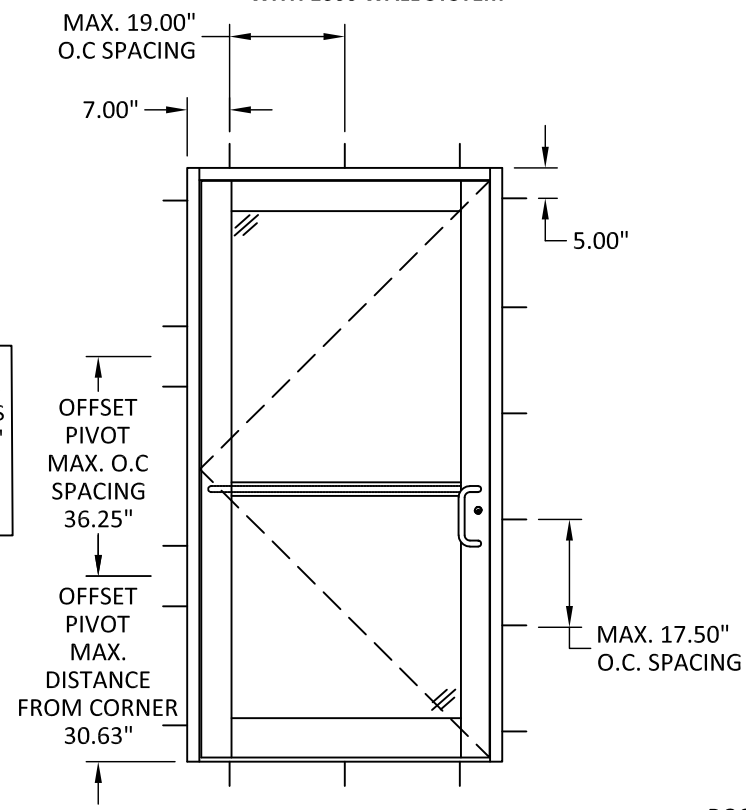
ANCHOR LAYOUT 500T THERMAL DOOR WITH 451T SUBFRAME W/ BUTT HINGE
