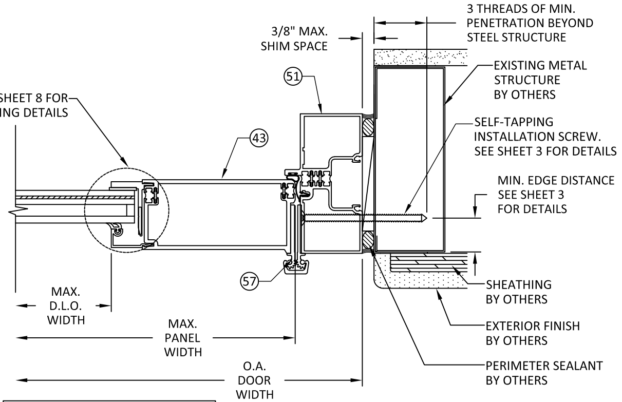
B HORIZONTAL SECTION 7 500T DOOR & TRIFAB 451T SUBFRAME JAMB-METAL STRUCTURE
