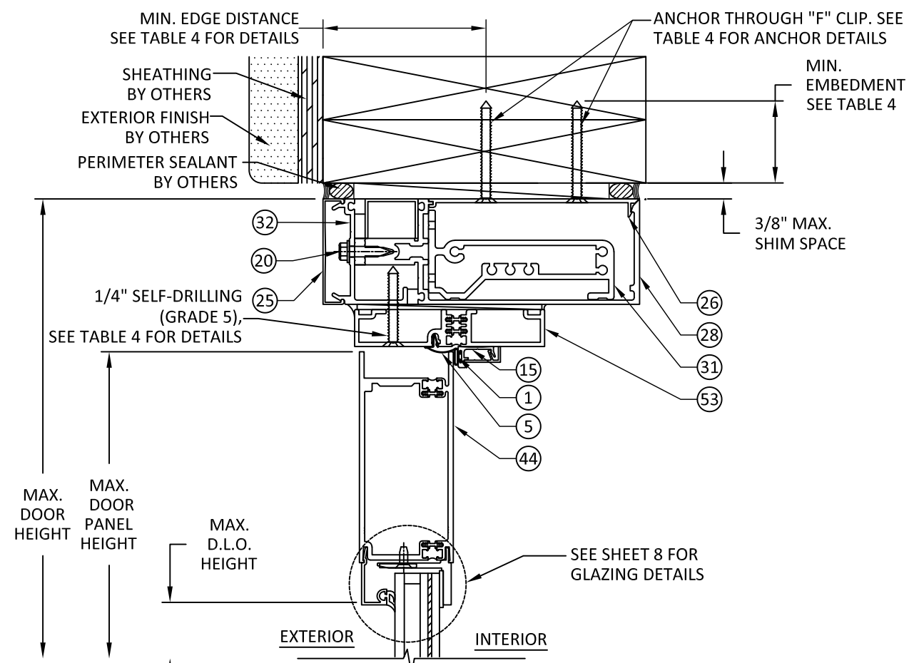
A 5 VERTICAL SECTION 500T DOOR & 1600 WALL SYSTEM HEAD - 2X WOOD FRAME
