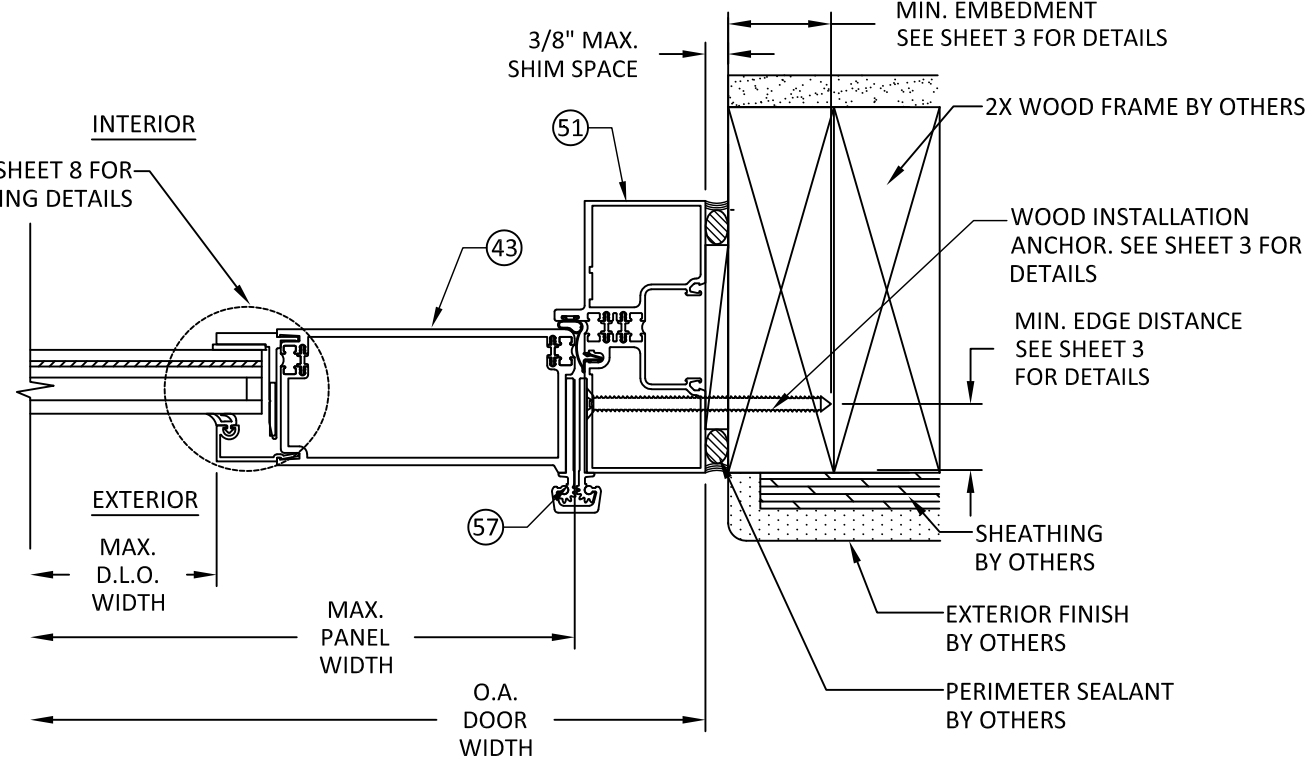
D HORIZONTAL SECTION 6 500T DOOR & TRIFAB 451T SUBFRAME JAMB-2X WOOD BUCK
