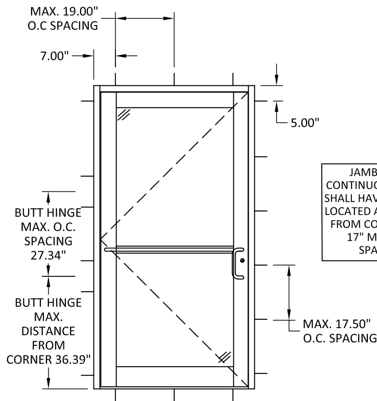
ANCHOR LAYOUT 500T THERMAL DOOR WITH 451T SUBFRAME W/ BUTT HINGE
