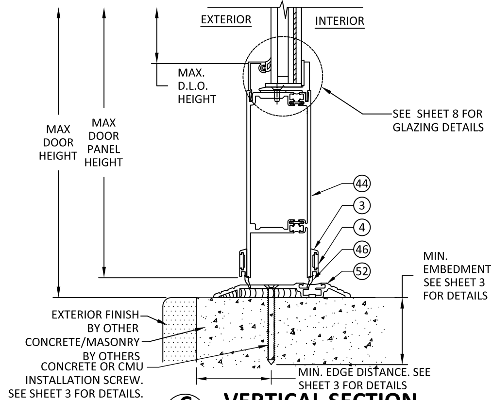
C 4 VERTICAL SECTION 500T DOOR & TRIFAB 451T SUBFRAME SILL - CONCRETE/MASONRY
